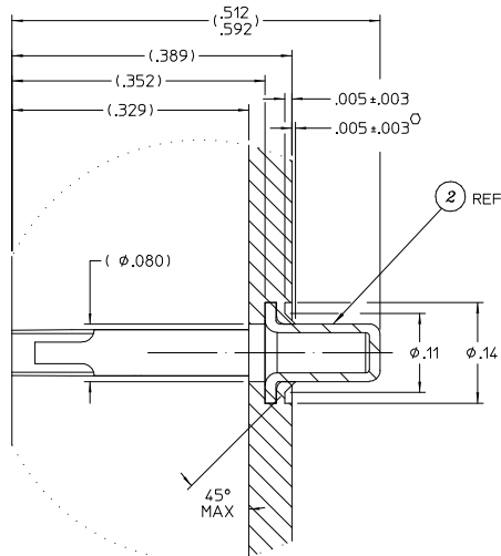
DETAIL E Scale 10:1
