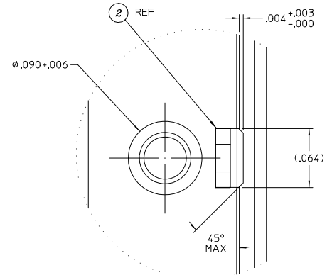
DETAIL J Scale 20:1
