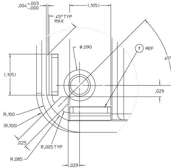
DETAIL H Scale 20:1
