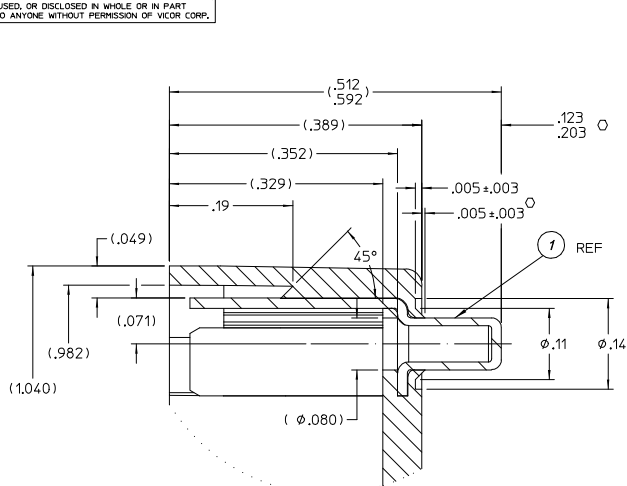
DETAIL D Scale 10:1
