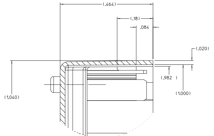
DETAIL F Scale 10:1
